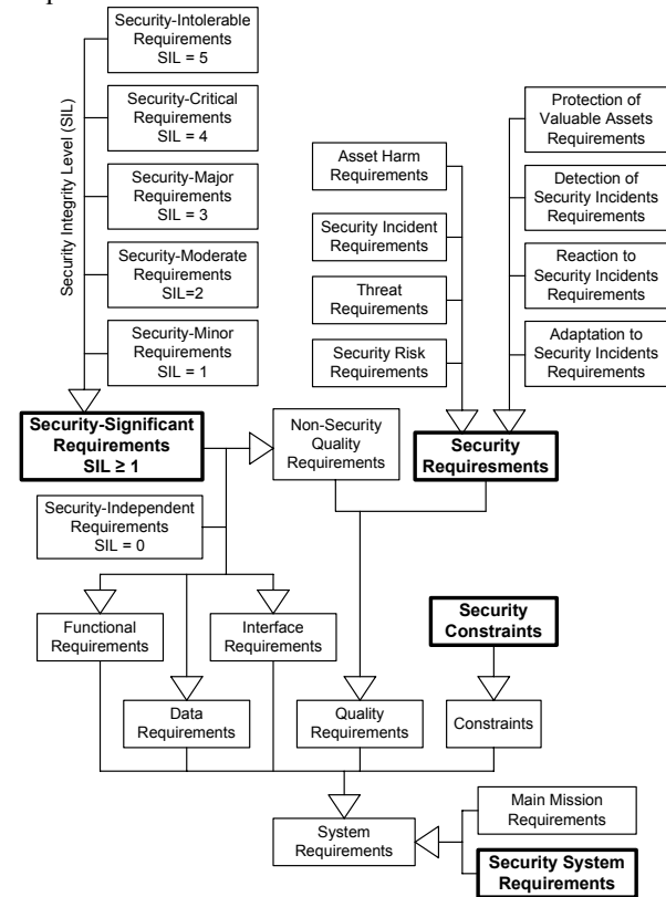
Figure 11: Taxonomy of Security-Related Requirements
